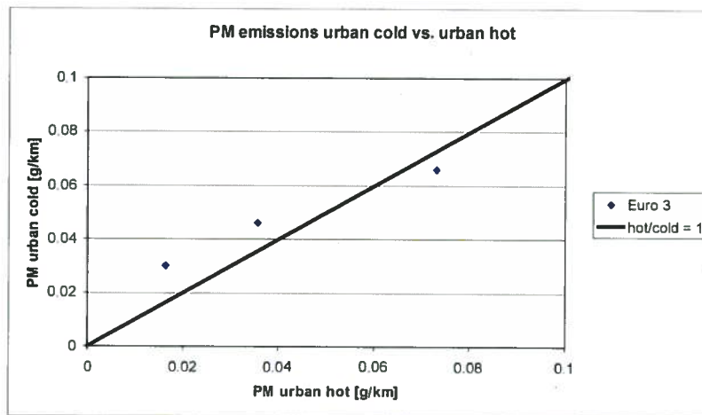
Figure 21: Diesel UDC cold start emissions versus UDC hot start emissions: PM
