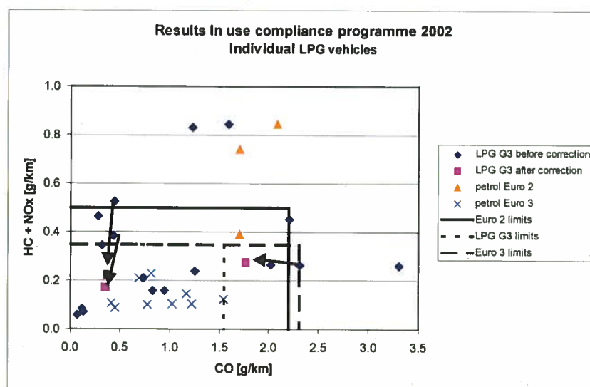
Figure 24: Results of individual in-use LPG passenger cars during the standard type approval test procedure
