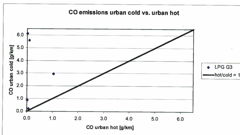
Figure 27: LPG UDC cold start emissions versus UDC hot start emissions: CO
