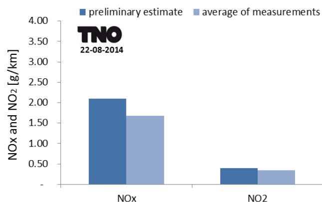
Figure 16: Comparison of the average \text{NO}_x (left) and \text{NO}_2 (right) emission test results with the preliminary estimated average emission level scenario that was input for the projections on future air quality in Utrecht [Utrecht, 2013]
