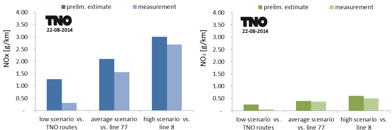
Figure 15: Comparison of the \text{NO}_x (left) and \text{NO}_2 (right) emission test results with the preliminary estimated emission level scenarios that were input for the projections on future air quality in Utrecht [Utrecht, 2013]
