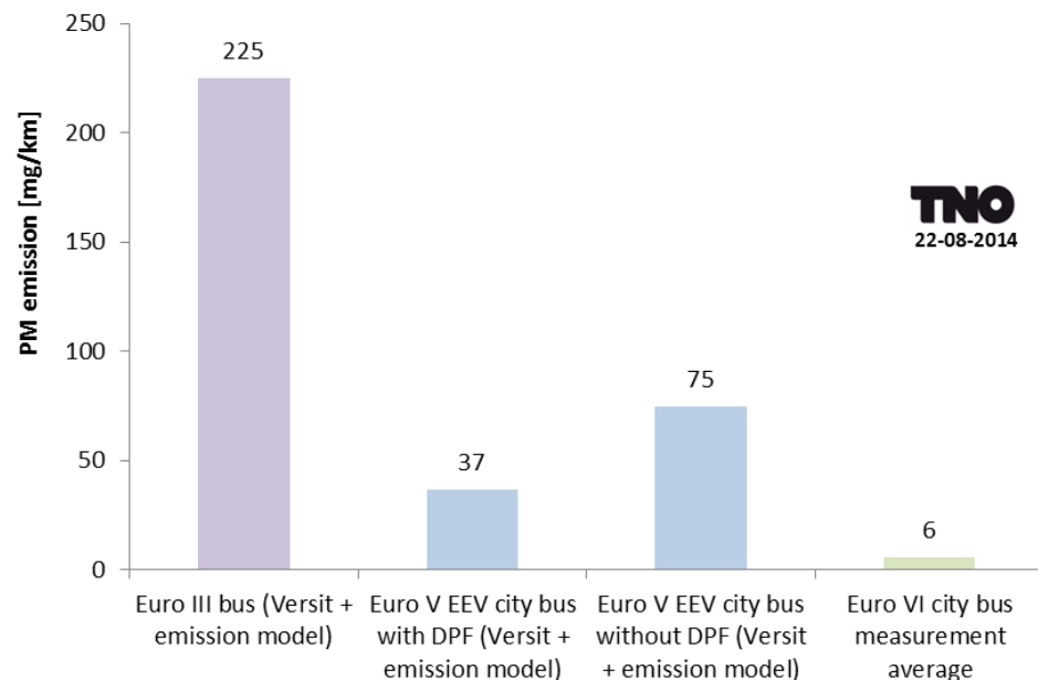
Figure 13: Comparison of the average PM emissions of the Mercedes Citaro with the emission factors for city operation, calculated by the Versit+ emission model [Hensema, 2013], for a Euro III city buses and a Euro V EEV city bus with and without Diesel Particulate Filter (DPF).
